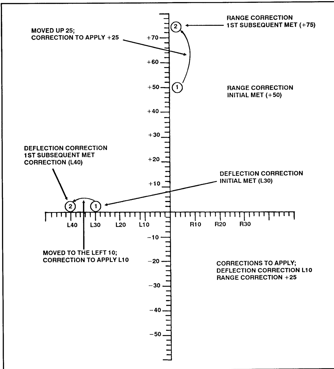
Figure 4-25. Deflection and range corrections.
