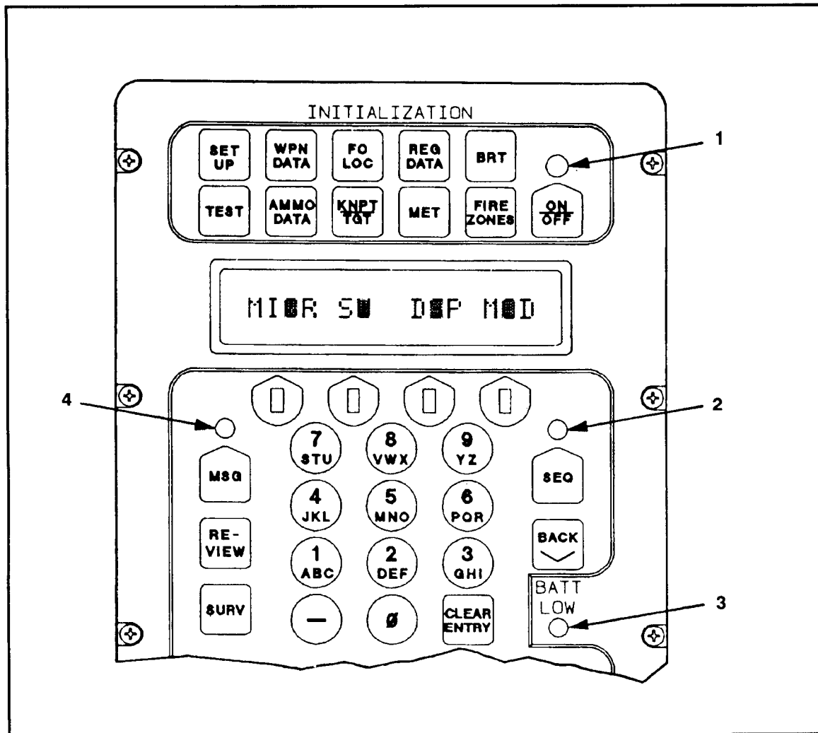
Figure 6-8. LED indicators.
