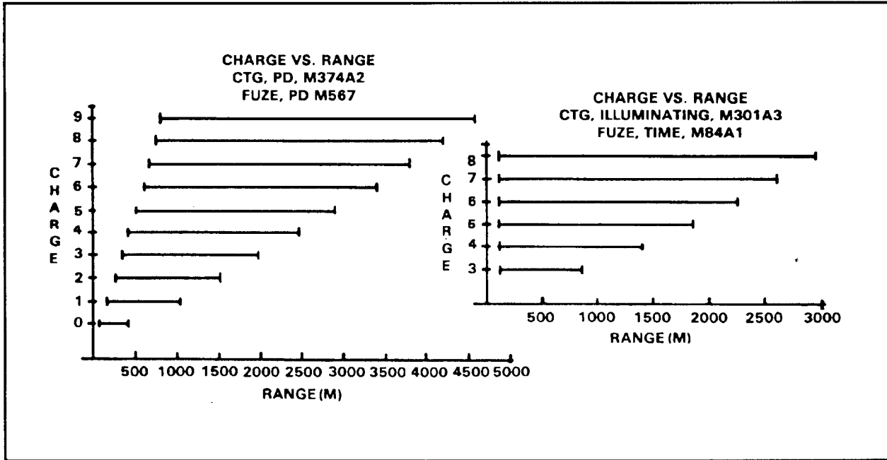
Figure 12-4. Charge-vs-range chart.
